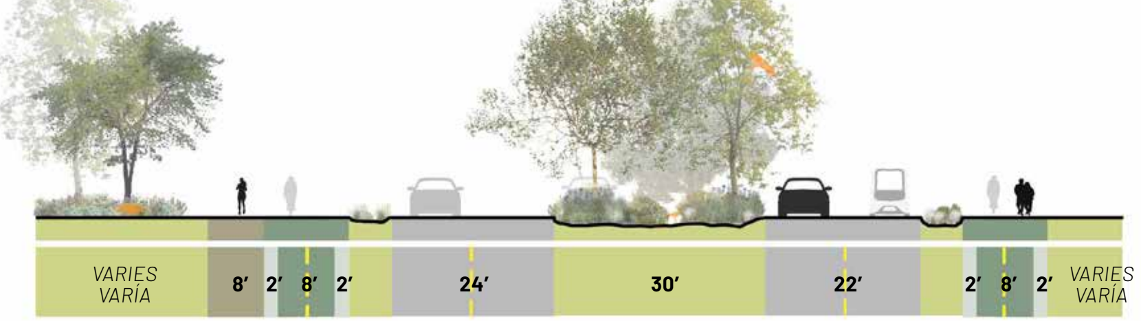
BURBANK BLVD PROPOSED COMPLETE STREET
