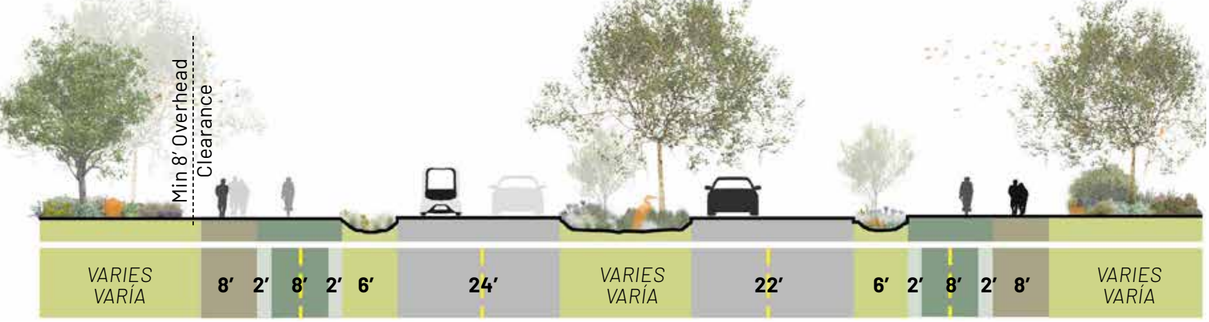
BALBOA BLVD PROPOSED COMPLETE STREET
