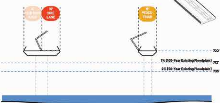
SECTION C / CORTE C
