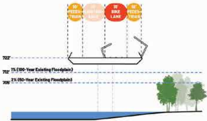
SECTION B / CORTE B
